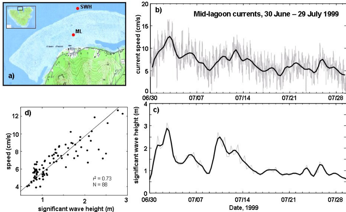
Figure 3. Time series from summer 1999 show dependence of current speed on significant wave height (SWH) at a reef on the north shore of Moorea. (a) Inset and small rectangle show study area on Moorea. Larger map of study area shows locations of bottom pressure sensor for estimating SWH (red circle labeled SWH) and mid-lagoon current meter (red circle labeled ML). (b) Time series of current speed at ML every 10 min (gray line) and smoothed with 36-hour low pass filter to remove tides (black line). (c) Time series of SWH measured every eight hours (gray line) and smoothed with 36-hour low pass filter (black line). (d) Scatter plot shows clear relationship between SWH and current speed at ML. Correlation between SWH and current speed is significant with r^2 = 0.73 . Other processes such as variable wave direction and wind forcing may account for the scatter between current speed and SWH. (Washburn, Holbrook & Schmitt unpub. data)
